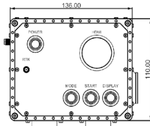
LEFT VIEW
