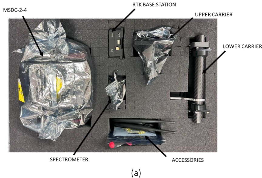
Figure 3. (a) MSDC-2-4 system package and its contents, (b) waterproof equipment case.
