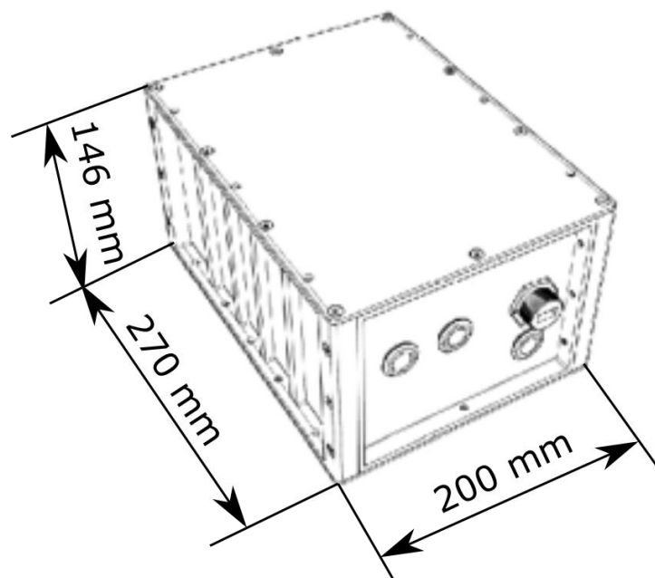
Control box
